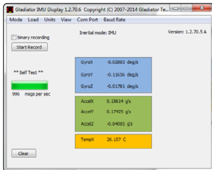
IMU Data in Full Mode at 1kHz Data Rate
